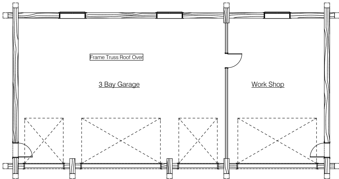
Main Floor
