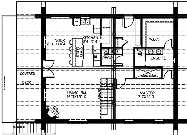
MAIN FLOOR AREA: 1280 SQ.FT.
